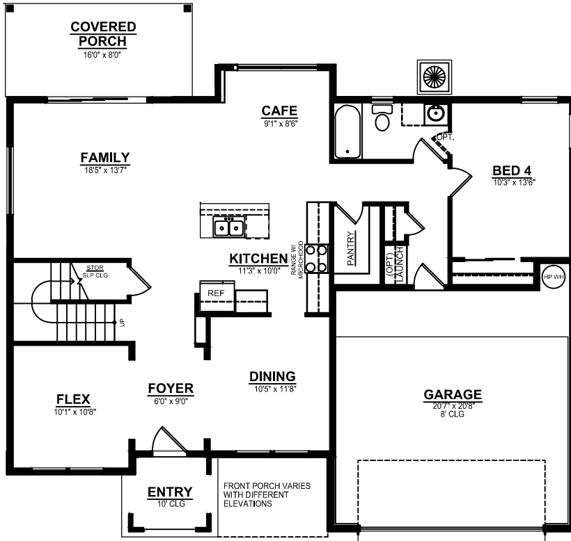
1st FLOOR 9' CEILINGS
